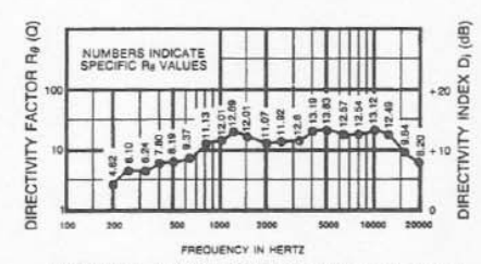
FIGURE 4 - MTH-2/94A Directivity Factor and Directivity Index vs. Frequency Response (composite of both orientations)
